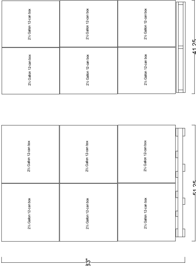
2½ Gallon Pallet Stacking 144 cans - 12 cases - 364 lbs. - 100.87 cubic ft.
